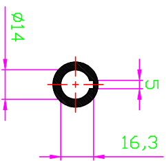
VIEW "J"
