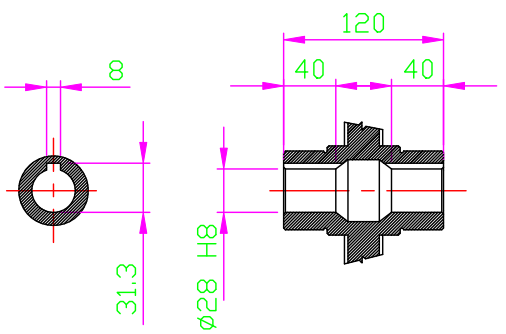
OUTPUT HOLLOW SHAFT
