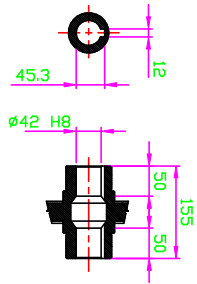
OUTPUT HOLLOW SHAFT
