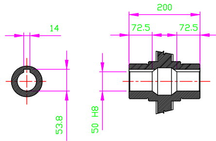
OUTPUT HOLLOW SHAFT
