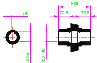
OUTPUT HOLLOW SHAFT
